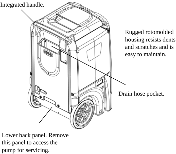
FIG. D: PUMP ACCESS PANEL
