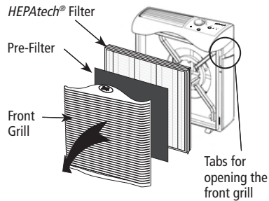
Figure 2 - Models 30212 & 30213
