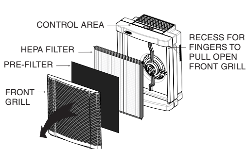
Fig. 2 - Air Purifier Components
