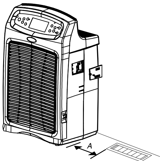
A. 6" (15.2 cm) minimum clearance
