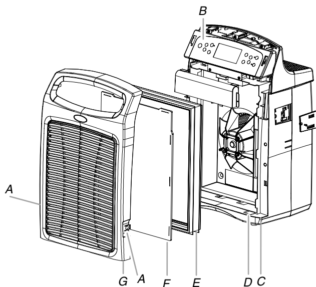
A. Release tabs D. Bottom slot F. Pre-filter B. Control panel E. HEPA filter G. Front grille C. Mainframe assembly
